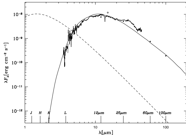
Fig. 1. Observed and modelled spectral energy distribution. The dot represents the near infrared and IRAS photometric results and the thin solid line is the ISO-SWS spectrum starting from band 1E. The flux at 15 micron measured from the ISO-CAM LW3 image is given by an open circle. The thick line is calculated from the model with the values of the parameters listed in Table 1 and the long-dashed line represents the radiation spectrum from the central star which radiates as a blackbody of temperature 2500 K.
